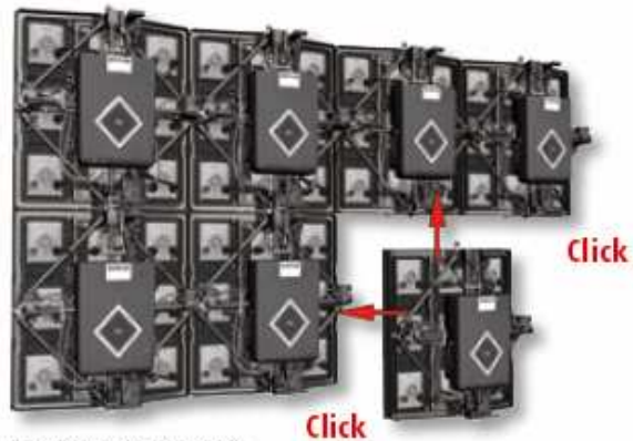
Ease of setup using click pre-locks
